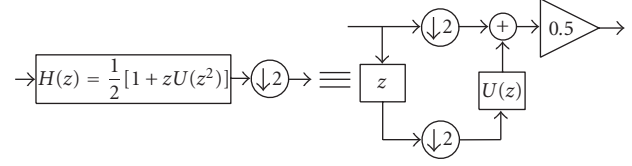
FIGURE 3: Lifting update implementation of a halfband filter.
